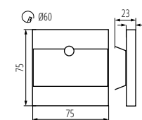
TERRA LED PIR B
