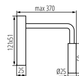
TONIL II LED
