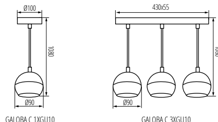
GALOBA C 1XGU10
