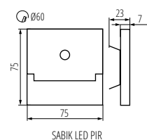
SABIK LED PIR
