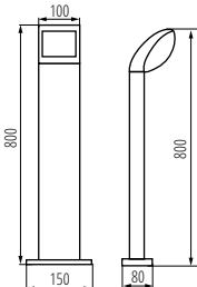
ABETE LED 80 GR
