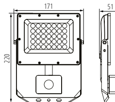
ACETE 30W CCT GR
