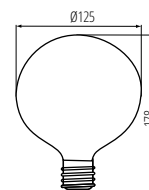
XLED G125, XLED G125C
