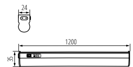
MER LED 15W CCT
