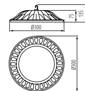
HIBO LED N 100W
