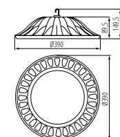
HIBO LED N 150W
