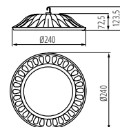
HIBO LED N 50W
