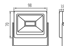
GRUN V3 LED-10-B
