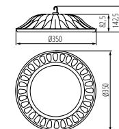
HIBO LED N 150W
