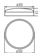
DUNO LED N24W
