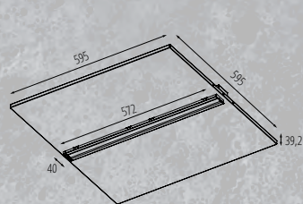
KN-P1
