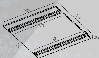
KN-P1D
