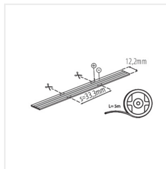
LCOB2L 28W/M24IP65-CW
