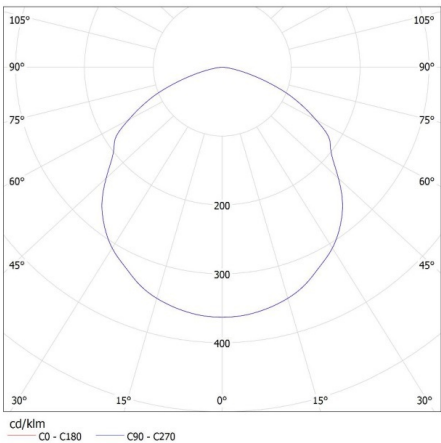
KANLUX S.A. (kat 27155+33193) HB PRO LED HI 100W-NW + LENS 120D / LDC (Polar)
