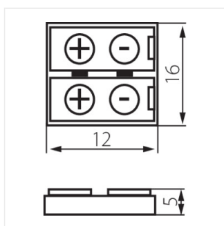
CONNECTOR 8
