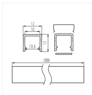
PROFILO F SET-MI-AL
