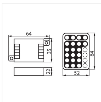
CONTROLLER RGB-IR20
