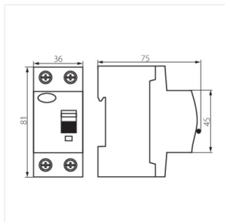
KRD6-2/25/300
