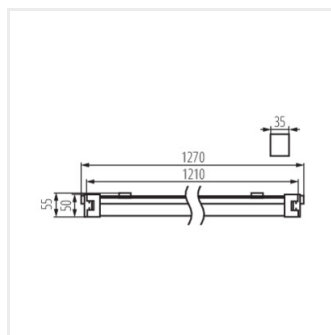
TP SLIM TW LED 40W-NW
