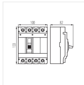
KMCCB-F-125A-4P
