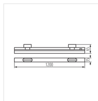
LTL-E 24W-120-CCT-B
