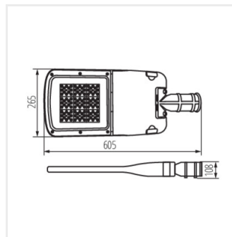
PRO-S M 105W NW
