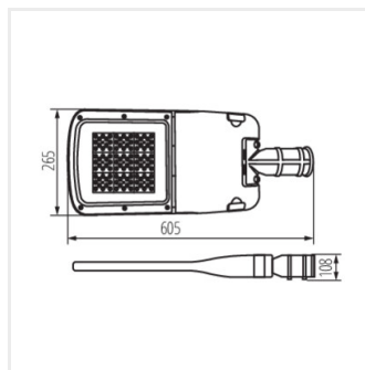
PRO-S M 110W NW
