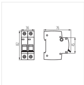
KMB10-B50/2
