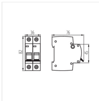
KMB10-B16/2
