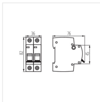
KMB10-B63/2
