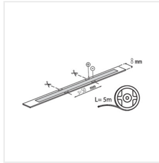
LCOB 8W/M 24 IP00-NW
