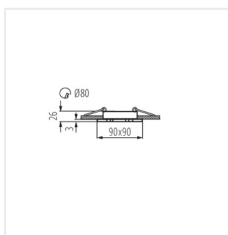
SEIDY CT-DTL50
