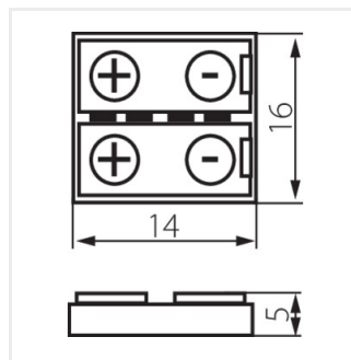
CONNECTOR RGB 10
