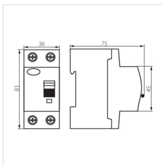
KRD6-2/25/100
