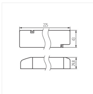
LC 60W 24V SC SNC
