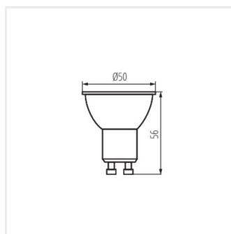
K LED GU10 6W
