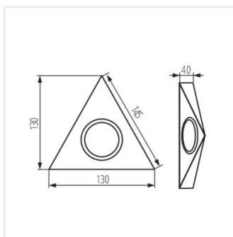
ZEPO LFD-T02/S-B
