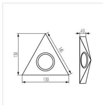
ZEPO LFD-T02/S-W
