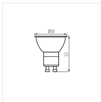
XLED GU10
