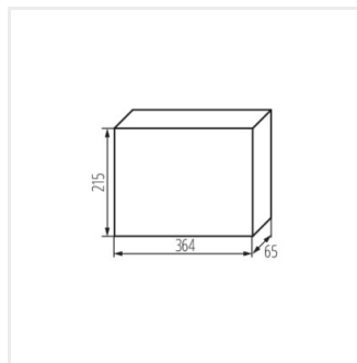
DB118F 1X18P/FMD-P
