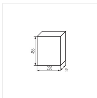
DB312F 3X12P/FMD-P
