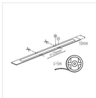
LCOB 14W/M 24IP00-CCT
