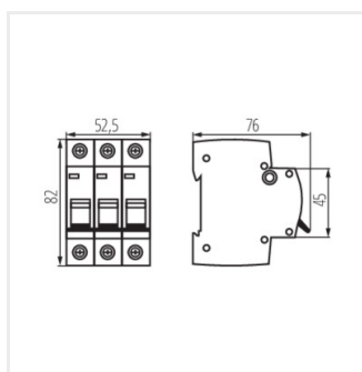
KMB10-C40/3
