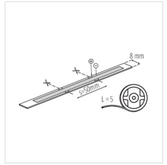
LC0B 3W/M 24 IP65-WW
