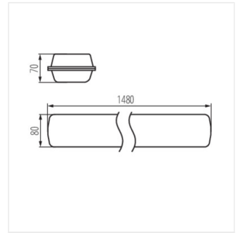
FT1200 55W-840
