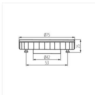
ESG LED 9W GX53-NW
