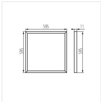
BRAVO PU36W6060NW W
