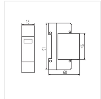
KSPD-T1T2 275/50 1P
