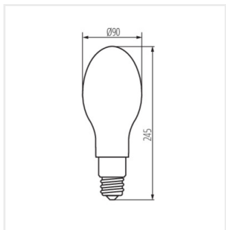
XLED HP D90E27 26W-NW
