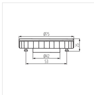
ESG LED 9W GX53
