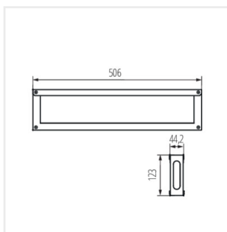
KP-DB-I-MF CON-H-L24
