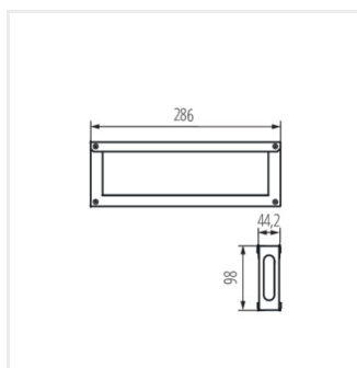
KP-DB-I-MF CON-H-S12
