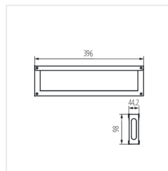
KP-DB-I-MF CON-H-M18
