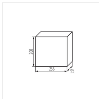
DB112S 1X12P/SMD-P
