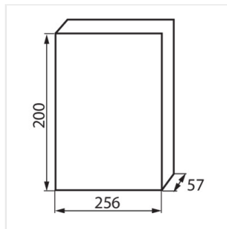
DB112F 1X12P/FMD
