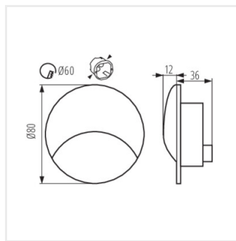
EXIN LED O
