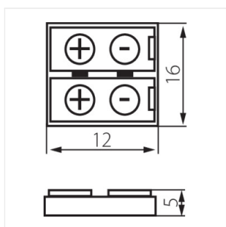
CONNECTOR 8
