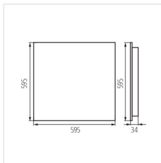
KNU-L9D-NW-W-P1D
