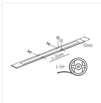
LCOB 14W/M 12IP00-CCT, 15:45 LCOB 14W/M 12IP65-CCT
