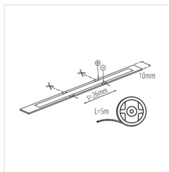
LCOB 14W/M 12IP00-CCT, 15:45 LCOB 14W/M 12IP65-CCT
