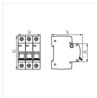
KMB10-B10/3
