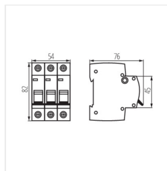
KMB10-B25/3
