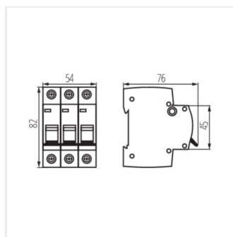
KMB10-B16/3
