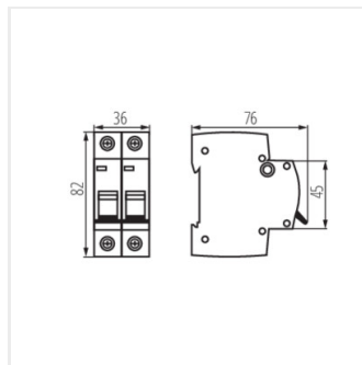
KMB10-B16/2
