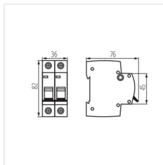
KMB10-B40/2
