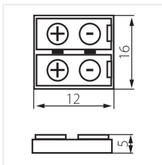
CONNECTOR 8
