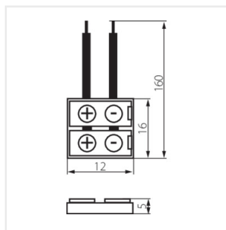
CONNECTOR 8-CP
