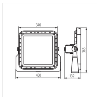
FLM LED 220W-...-60D; FLM LED 220W-...110-150
