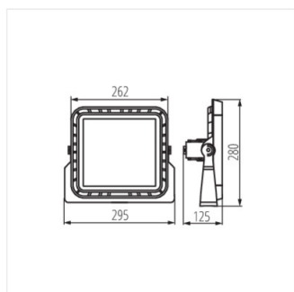
FLM LED 100W-...-60D; FLM LED 100W-...110-150
