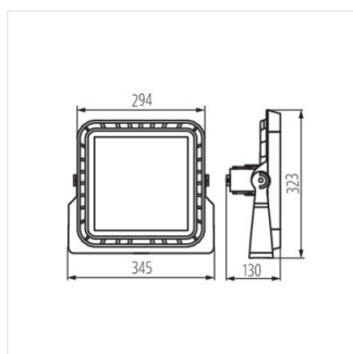
FLM LED 140W-...-60D; FLM LED 140W-...110-150
