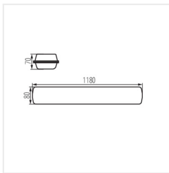
FTD1200 49W-840-OPL
