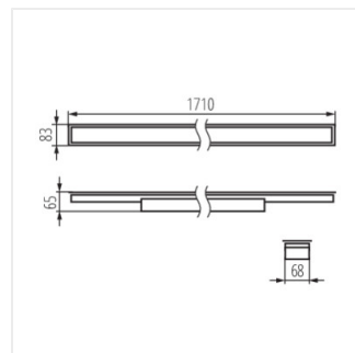
AL 35W-830-MAT-W-PT
