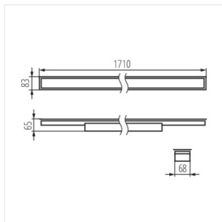
AL 35W-840-MAT-W-PT
