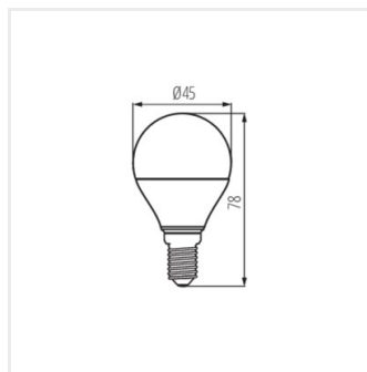
IQ-LED G45E14 4,2W
