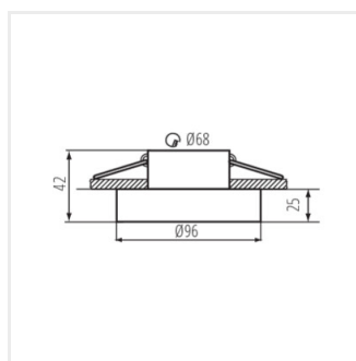
ELICEO-ST DSO
