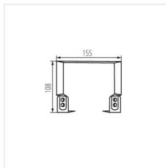
HBPHS BRACKET
