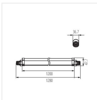
TP_SLIM_N-TN 40W
