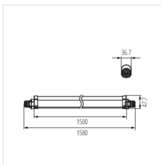
TP_SLIM_N-TN 50W
